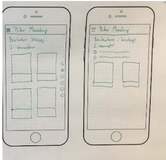
Lofi prototype
