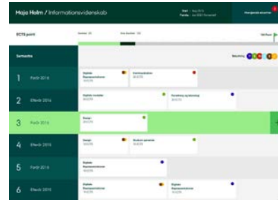
Hifi prototype
